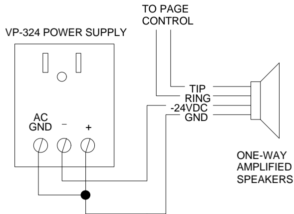
Connections to One-Way Amplified Speakers
